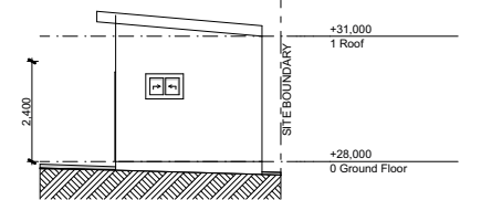
North Elevation 1:200
