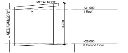
South Elevation 1:200
